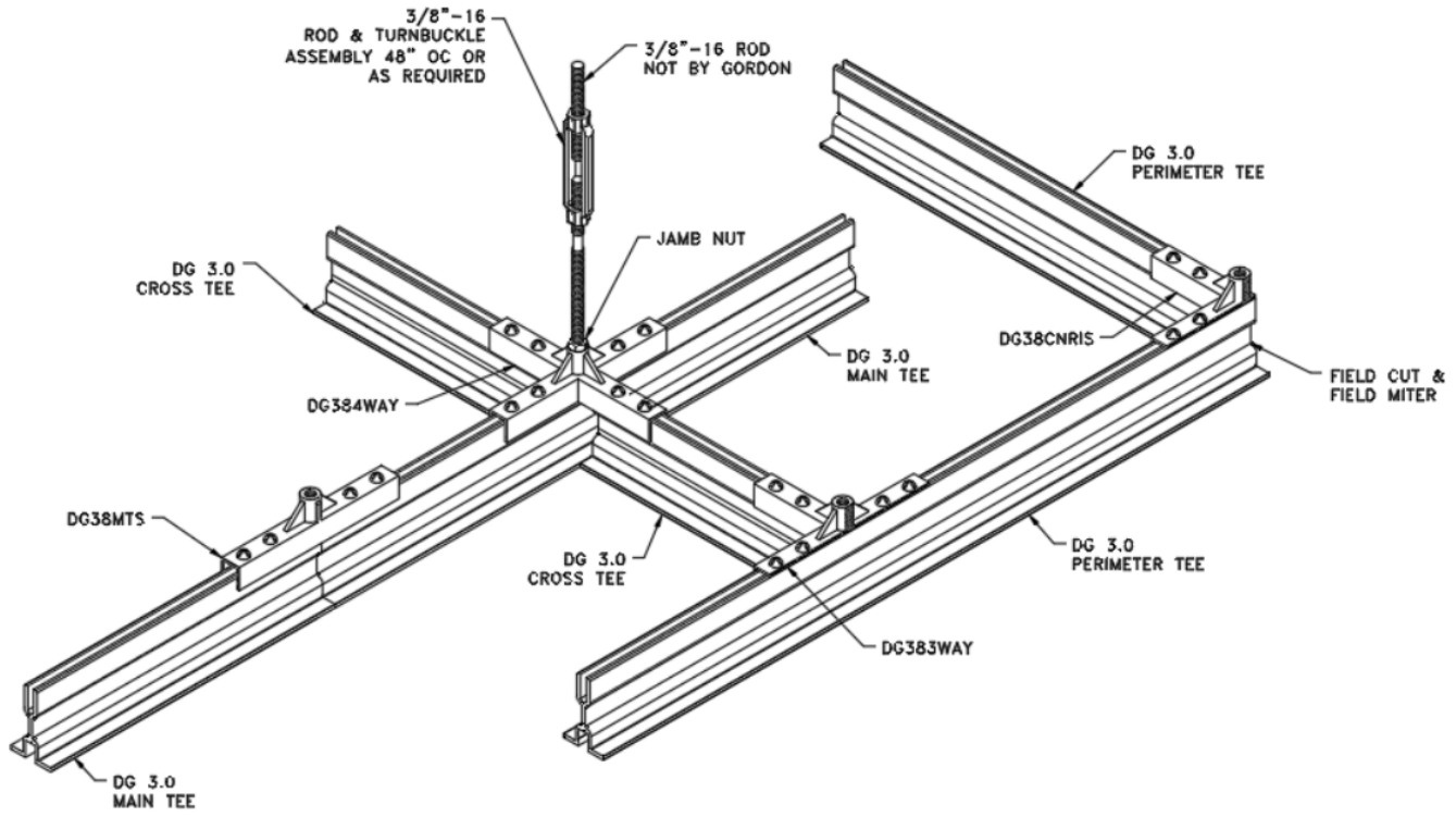
Figure B: DG Series Grid with Floating Perimeter Condition
