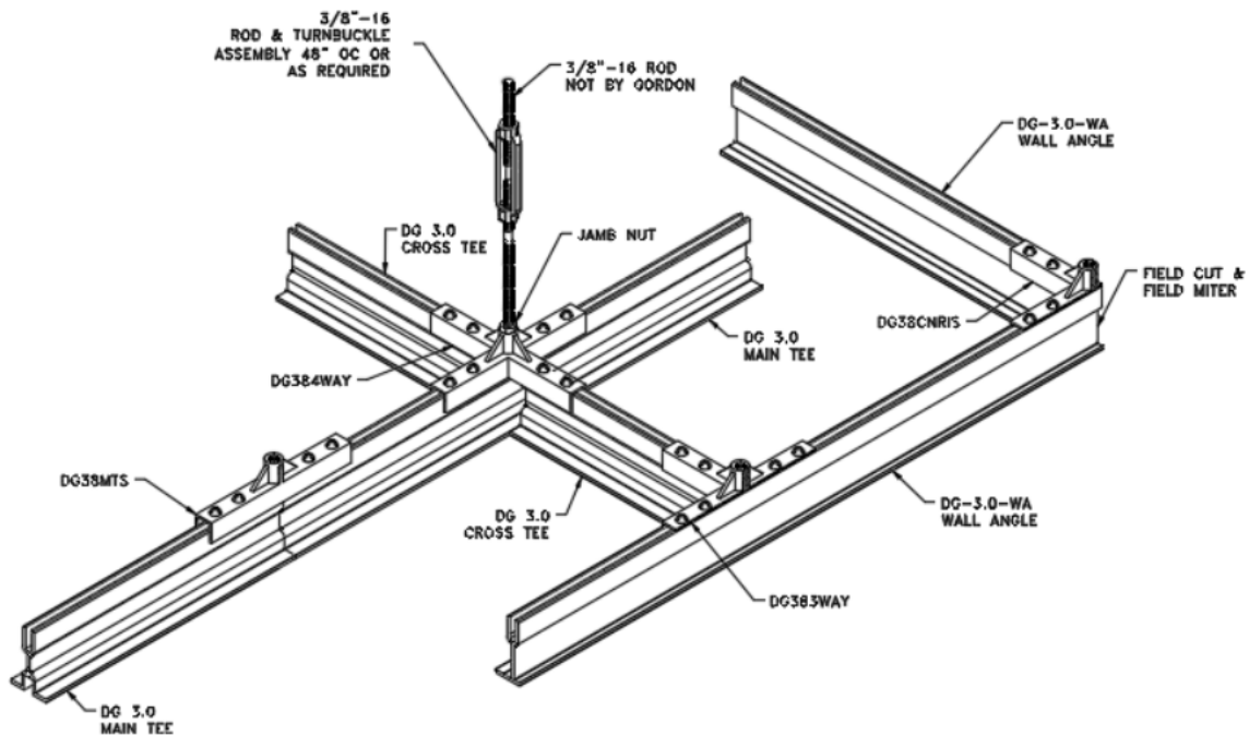
Figure A: DG Series Grid with Fixed Perimeter Condition
