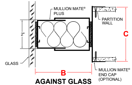
AGAINST GLASS
