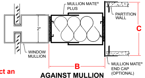
AGAINST MULLION
