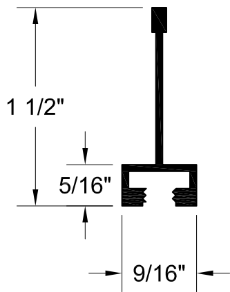
SERIES B SCREW SLOT: 5/16"-18
