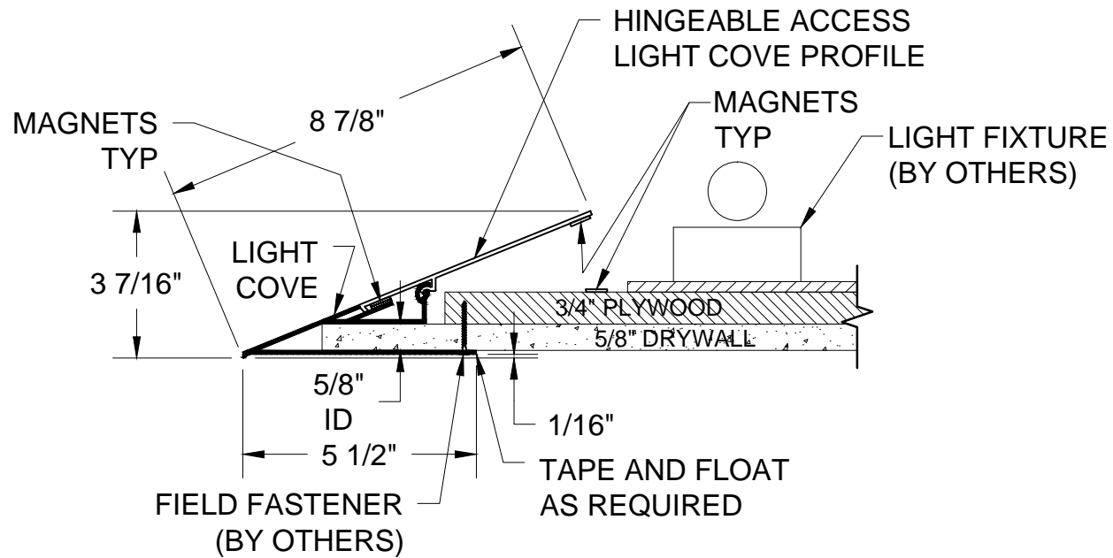
CLOSED POSITION
