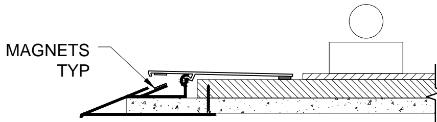
OPEN POSITION
