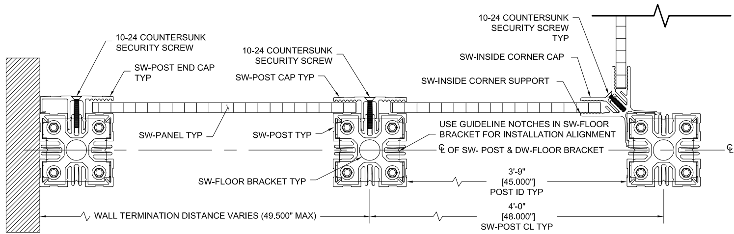
PLAN VIEW AT FLOOR
