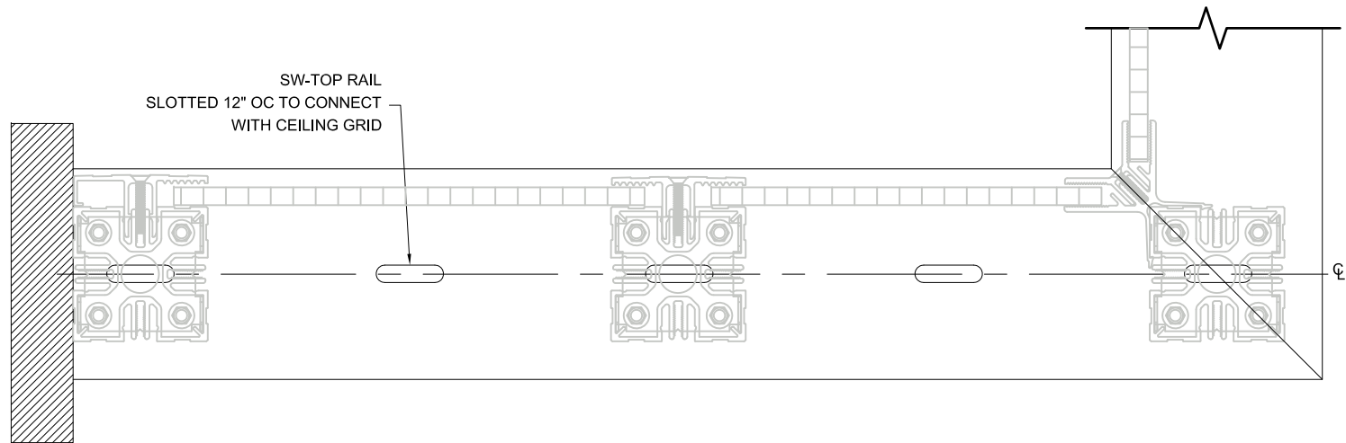
PLAN VIEW AT CEILING
