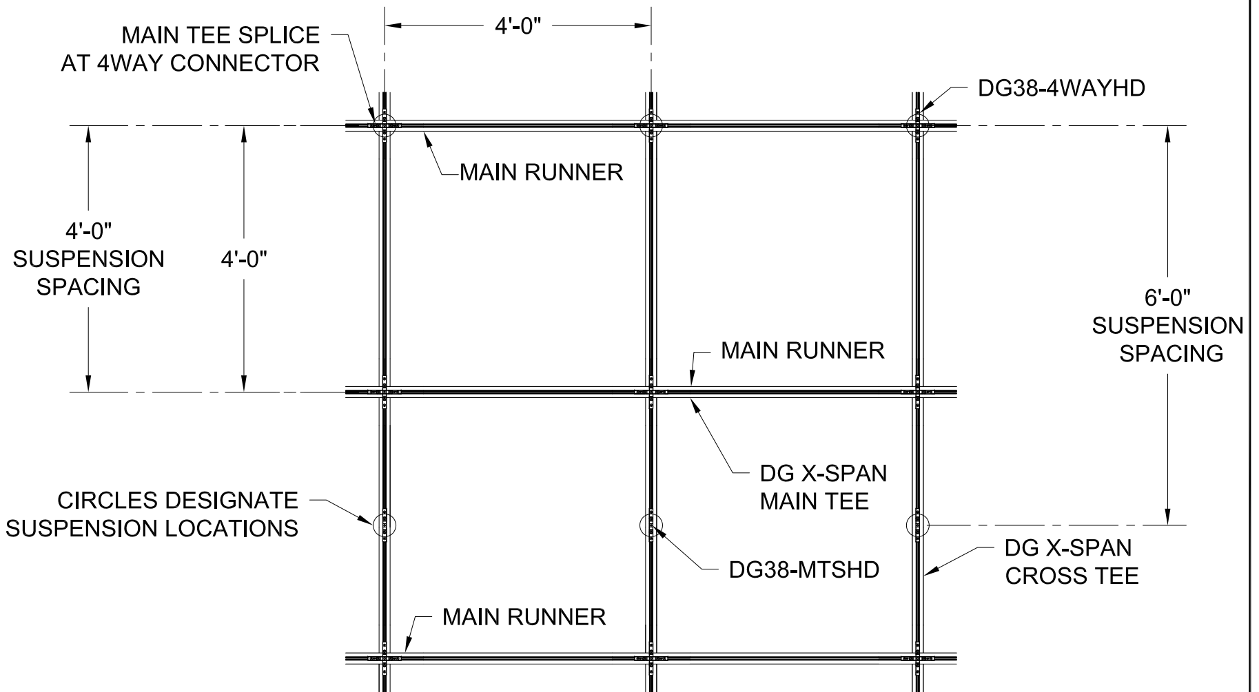
TYPICAL GRID PLAN NOT TO SCALE
