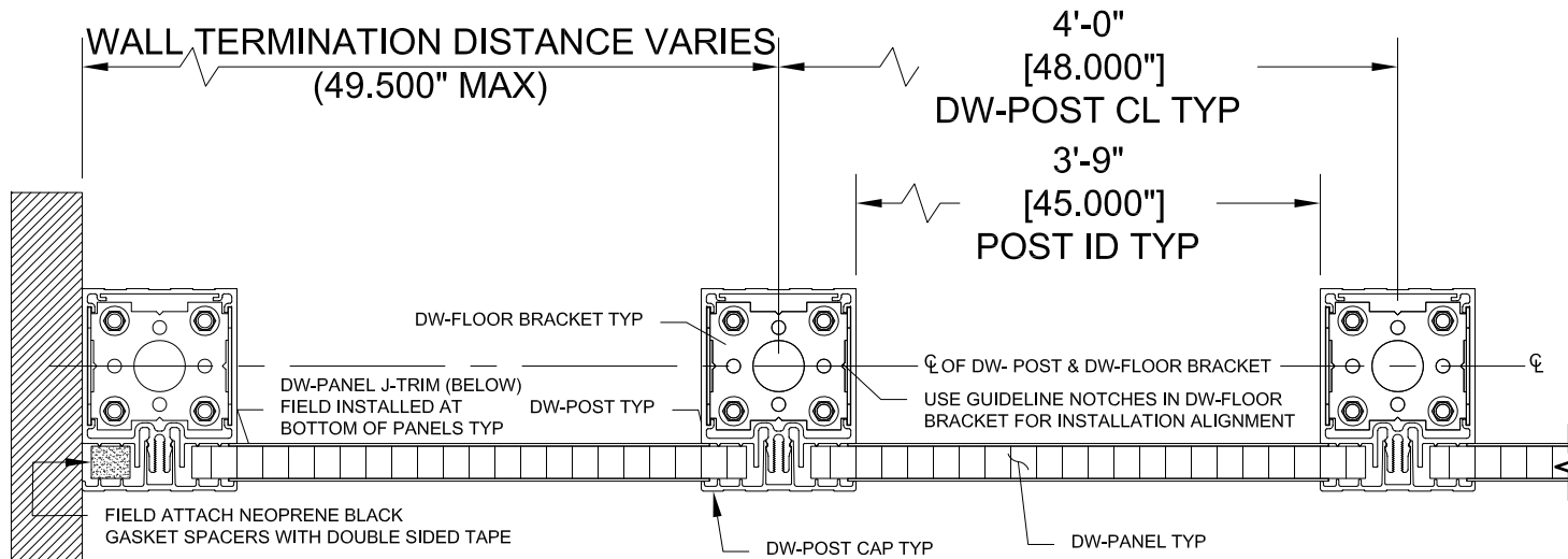
PLAN VIEW AT FLOOR
