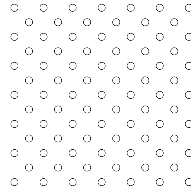
R564-732DG10 PANEL PERFORATION DETAIL 5/64" HOLES ON 7/32" 45° DIAGONAL CENTERS 10% OPEN AREA
