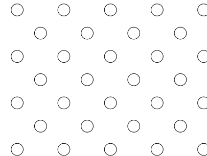
R18-1132DG11 PANEL PERFORATION DETAIL 1/8" HOLES ON 1 1/32" 45° DIAGONAL CENTERS 11% OPEN AREA
