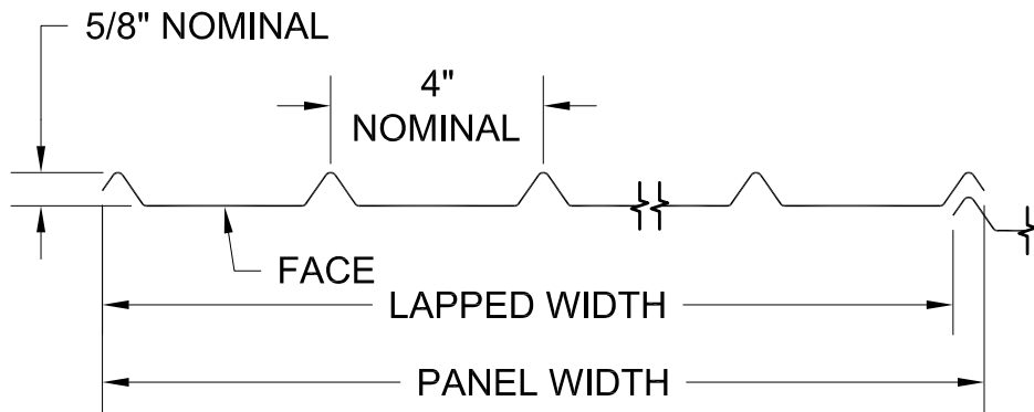
AI - ALUMINUM / STEEL MAXIMUM LENGTH: 120"
