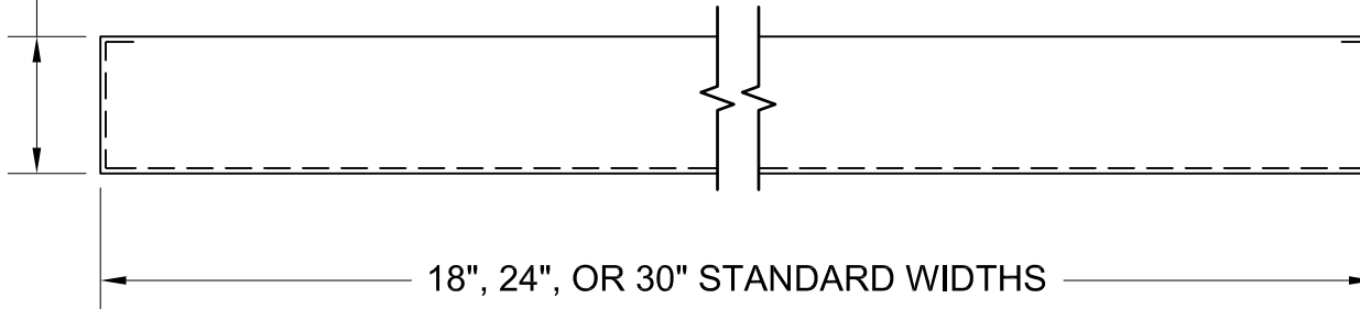
FLAT-BAF-I ALUMINUM / STEEL MAXIMUM LENGTH: 120"
