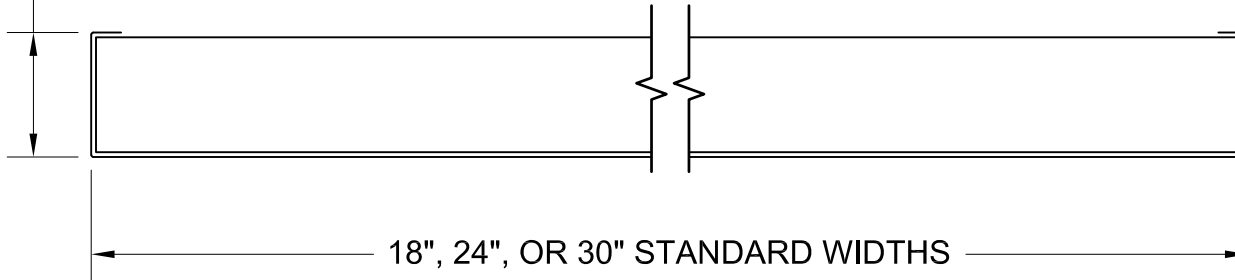
FLAT-BAF-O ALUMINUM / STEEL MAXIMUM LENGTH: 120"
