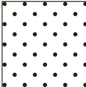
Item # R116-14DG05 Open Area: 5% Pattern: Round 1/16" (.063") x 1/4" (.250") Diagonal Centers
