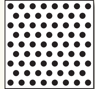
Item # R332-316SG23 Open Area: 23% Pattern: Round 3/32" (.094") x 3/16" (.188") Staggered Centers
