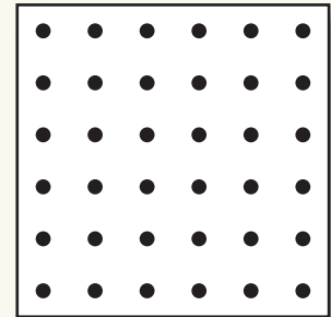
Item # R116-14ST05 Open Area: 5% Pattern: Round 1/16" (.063") x 1/4" (.250") Straight Centers
