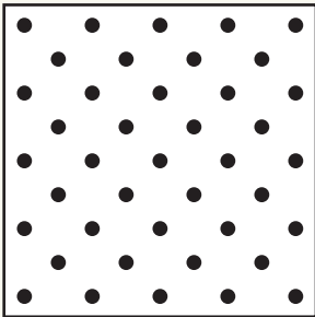
Item # R116-1564DG06 Open Area: 6% Pattern: Round 1/16" (.063") x 15/64" (.231") Diagonal Centers
