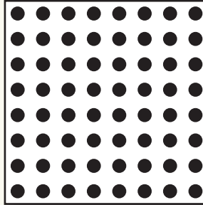
Item # R332-316ST20 Open Area: 20% Pattern: Round 3/32" (.094") x 3/16" (.188") Straight Centers
