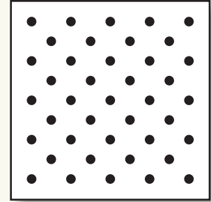
Item # R116-1364DG07 Open Area: 7% Pattern: Round 1/16" (.063") x 13/64" (.210") Diagonal Centers
