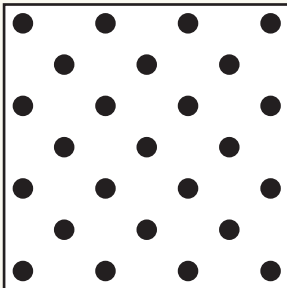
Item # R332-516DG08 Open Area: 8% Pattern: Round 3/32" (.098") x 5/16" (.307") Diagonal Centers
