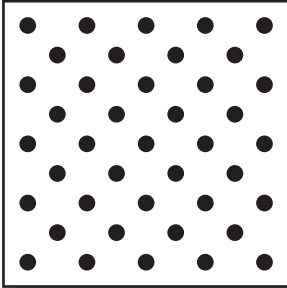
Item # R564-732DG10 Open Area: 10% Pattern: Round 5/64" (.078") x 7/32" (.220") Diagonal Centers
