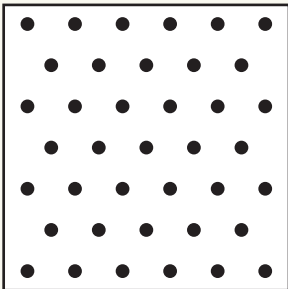
Item # R116-14SG06 Open Area: 6% Pattern: Round 1/16" (.063") x 1/4" (.250") Staggered Centers
