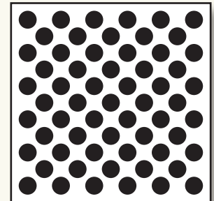
Item # R18-1164DG39 Open Area: 39% Pattern: Round 1/8" (.125") x 11/64" (.177") Diagonal Centers
