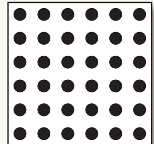
Item # R18-14ST20 Open Area: 20% Pattern: Round 1/8" (.125") x 1/4" (.250") Straight Centers
