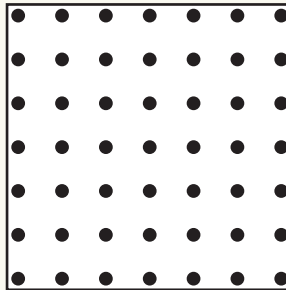
Item # R116-1564ST06 Open Area: 6% Pattern: Round 1/16" (.063") x 15/64" (.231") Straight Centers
