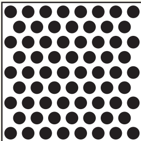
Item # R18-316SG40 Open Area: 40% Pattern: Round 1/8" (.125") x 3/16" (.188") Staggered Centers
