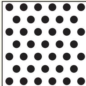
Item # R18-14SG23 Open Area: 23% Pattern: Round 1/8" (.125") x 1/4" (.250") Staggered Centers
