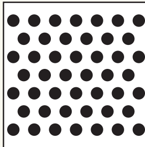
Item # R18-732SG27 Open Area: 27% Pattern: Round 1/8" (.118") x 7/32" (.216") Staggered Centers
