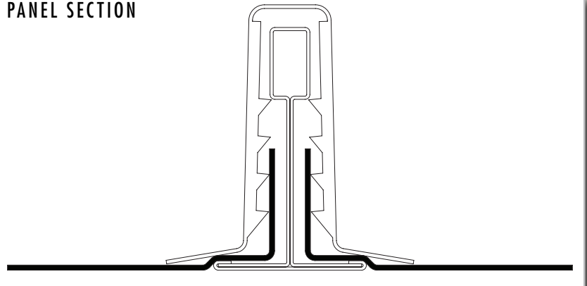
PANEL SECTION
