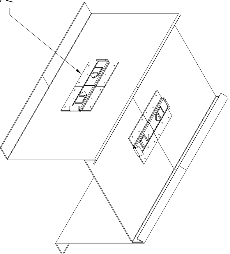
WELDED HANGER / SPLICE CLIP, TYP
