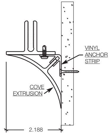
TYPICAL CEILING TRANSITION
